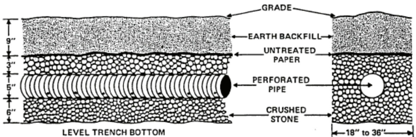
Figure 1. Construction details for an absorption trench
